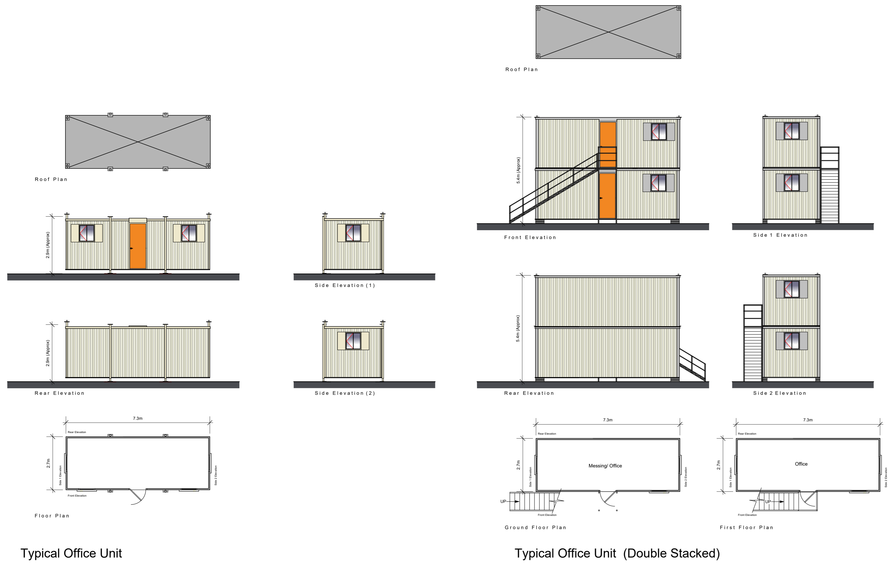
Central Site (West) - Typical Building Plans & Elevations / Enclosure and Associated Features
