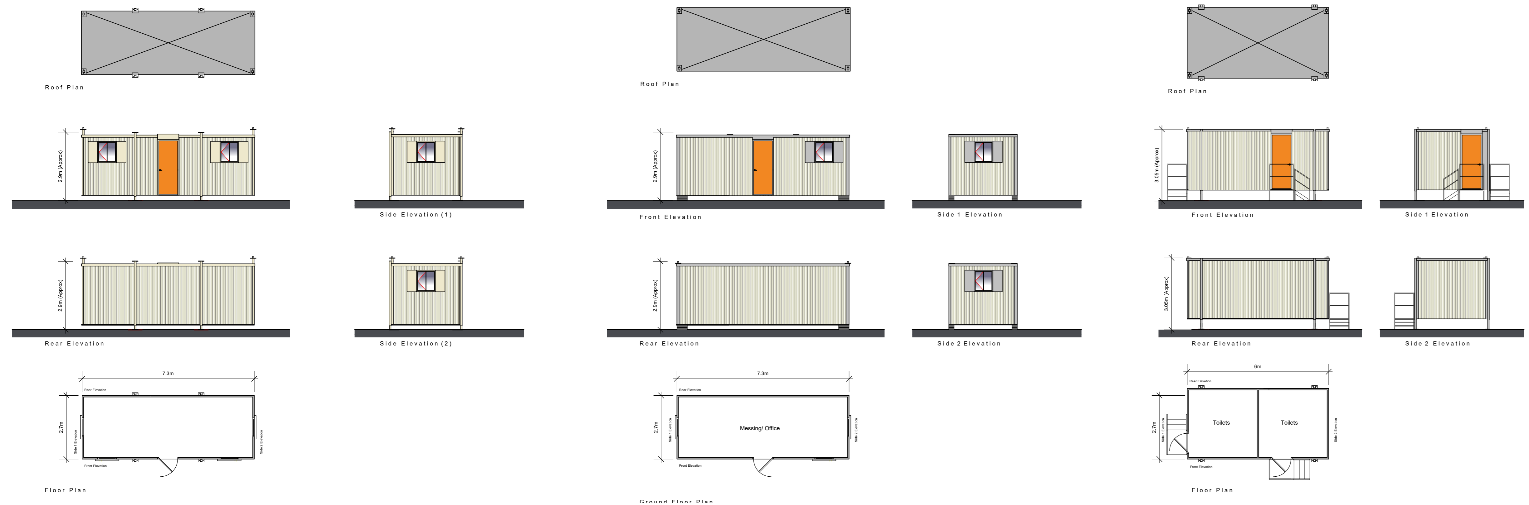
Typical Office Unit
