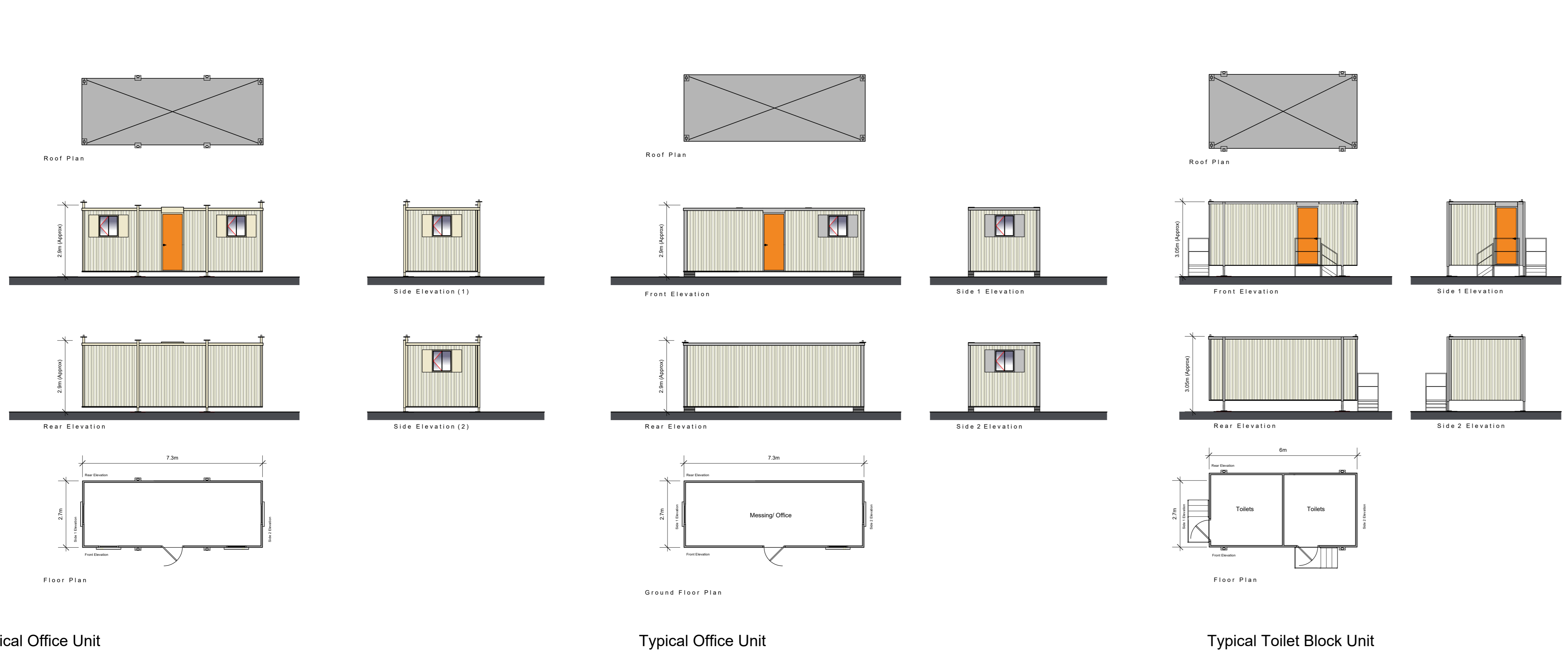
Central Site (East) - Typical Building Plans & Elevations / Enclosure and Associated Features
